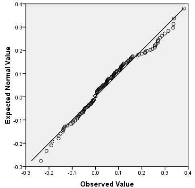
Normal Q-Q Plot of Return
