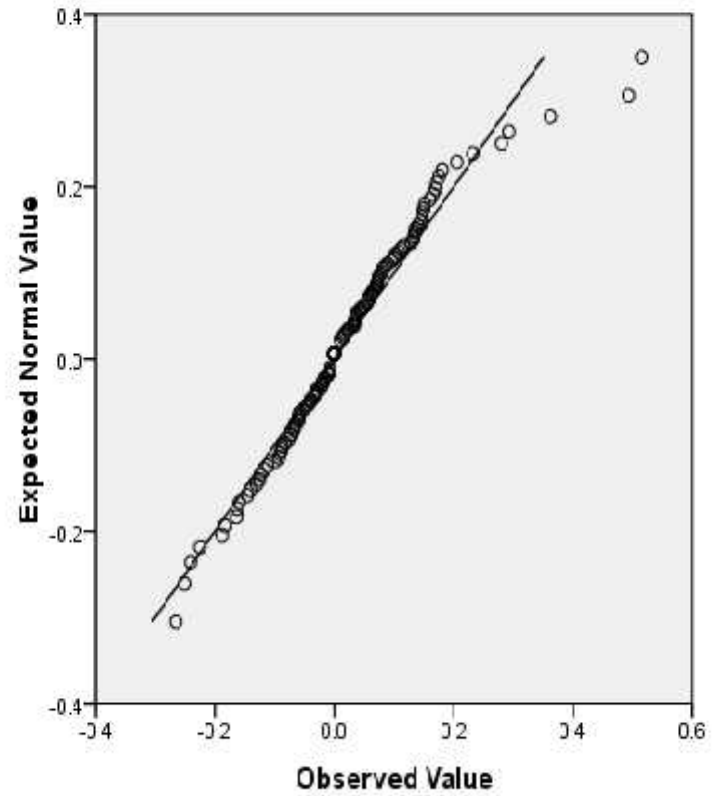
Normal Q-Q Plot of Return
