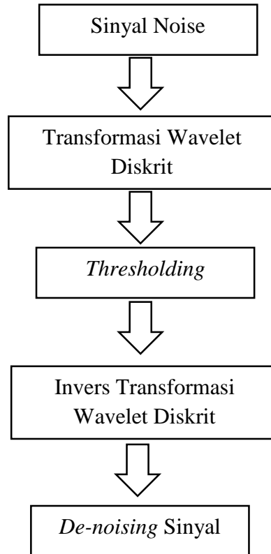
Gambar 3.3. Diagram blok de-noising sinyal
