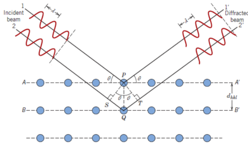
Gambar 2.3 Skema Hukum Bragg (Callister & Rethwisch, 2009).
